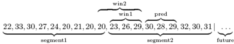
Figure 9: Window adaptation when analysis spans both segments. Note: win1 and win2 have contracted to include less inappropriate data.
