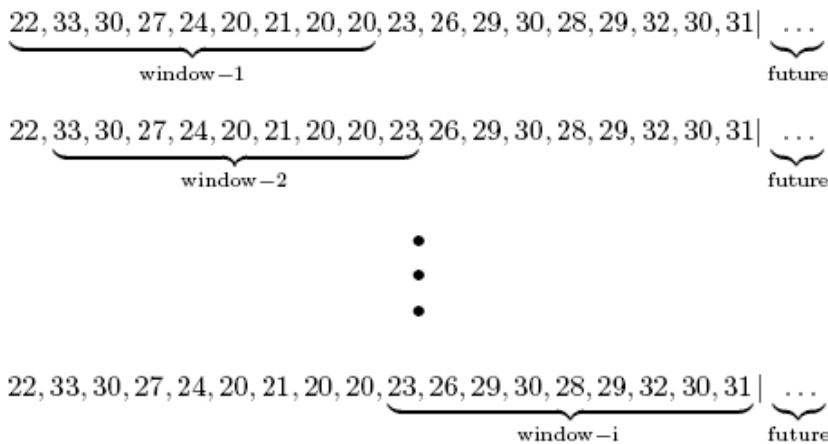
Figure 4: A sliding data analysis window.
