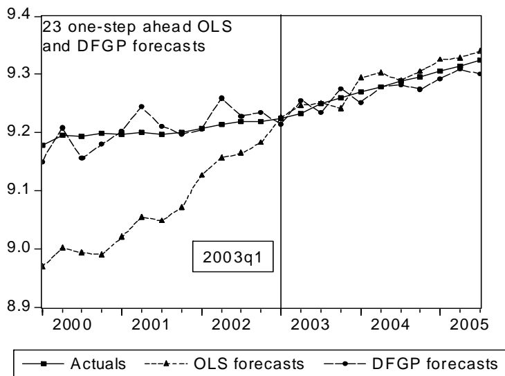
Figure 11: Actuals and OLS and DFGP forecasts
