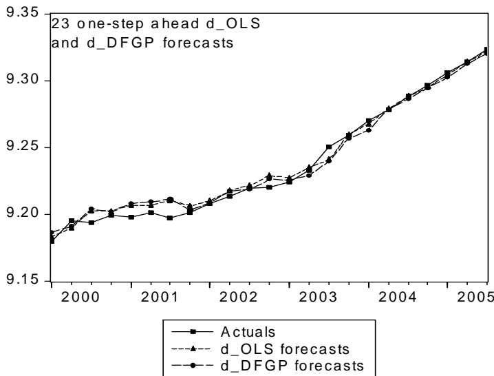
Figure 12: d_OLS and d_DFGP forecasts
